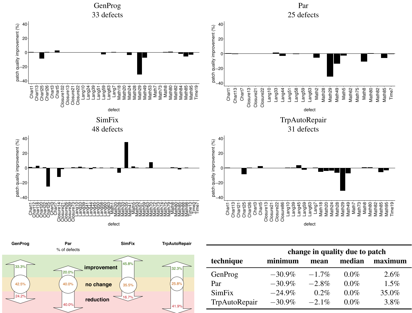
Fig. 5. Patch overfitting. Change in quality between the defective version and the patched version of the code. The median patch neither improves nor decreases quality. While more GenProg patches improve the quality than decrease it, the opposite is true for Par and TrpAutoRepair patches, and, on average, patches break more functionality than they repair. The data presented are for the 45 defects with high-quality evaluation test suites, of which GenProg produced patches for 33, Par for 25, and TrpAutoRepair for 31.
